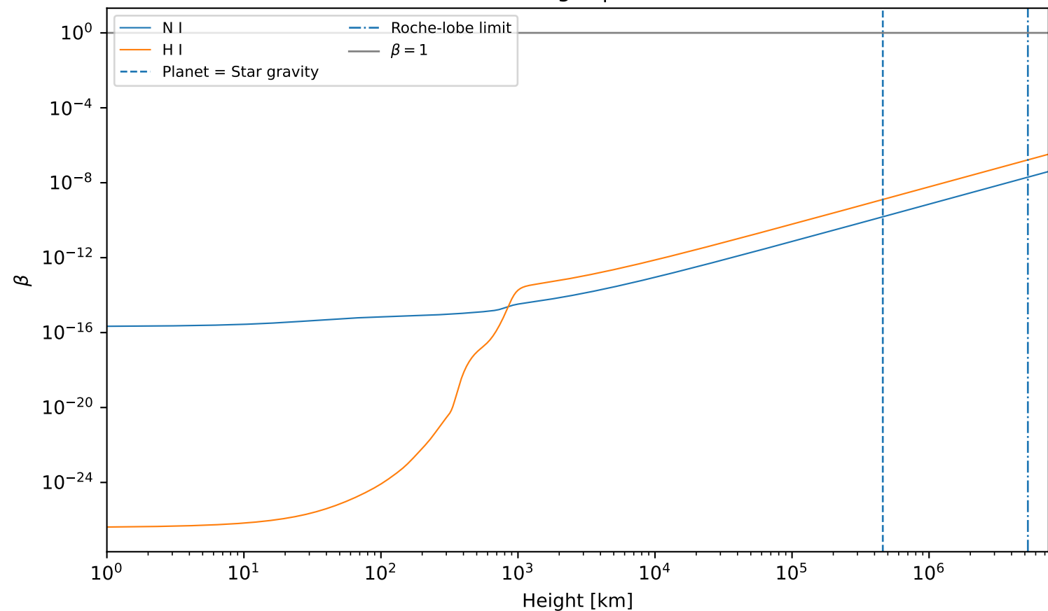
Beta vs height | Pluto-Sun
